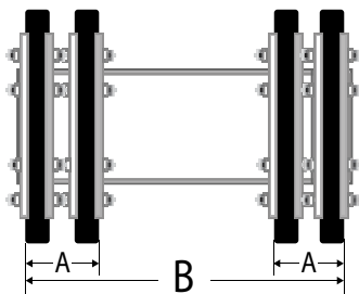
PRC-B4C-DNXXXX/STI Bidirectionnel
